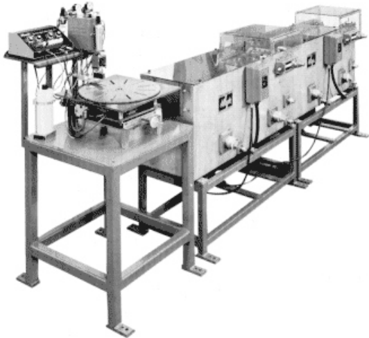
AM-30T - For marking tool bits with neutralizing and oiling tanks 1200-1400 P .P.H.
