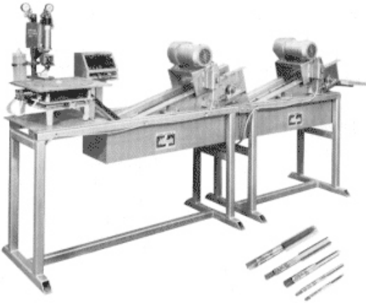
For marking drills, taps, reamers, or any small round, square, rectangular part .
