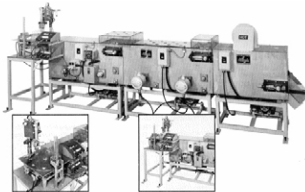
Modified AM-30T - To mark top and bottom at the same time. P arts are to be stack fed. Neotralizing tank, hot water rinse tank, and heated air tunnel fro complete drying of parts. Machine also has option for electronic pH meter which shuts down when pH falls below pre-determined number 1500 P .PH.
