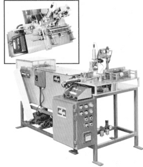
Bearing Marking Machine - Marks range from 2" to 6" on race or O.D . 1200-1400 P .PH.
