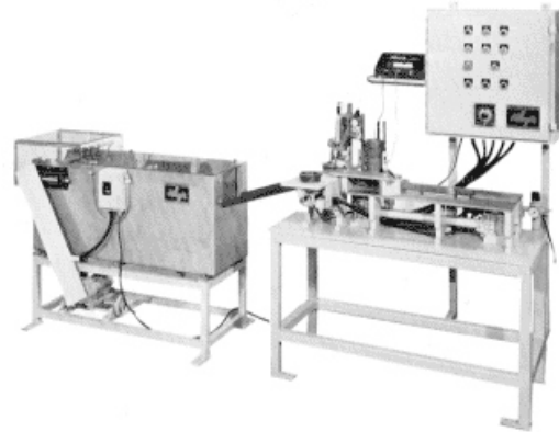
Bearing Marking Machine with Neutralizing Tank - Marks Face of bearings 2" to 6" range 1200-1400 P.P.H.
