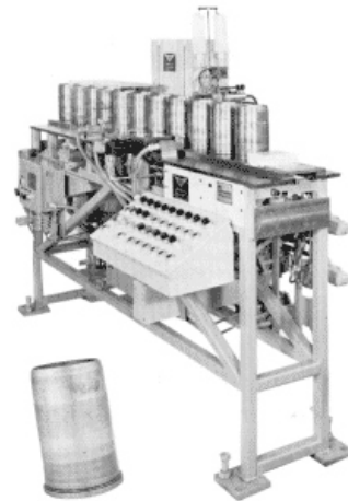
Bearing Marking Machine with Neutralizing Tank - Marks Face of bearings 2" to 6" range 1200-1400 P.P.H.
